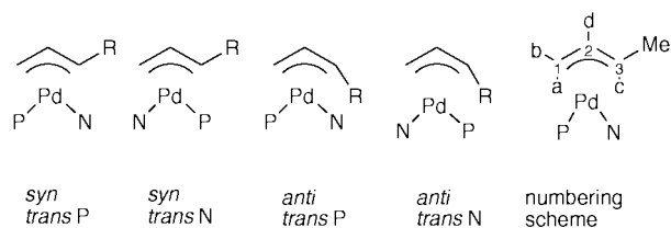
Fig. 3 Possible isomeric structures of cationic (C 4 H 7 )Pd(P-N) complexes.
